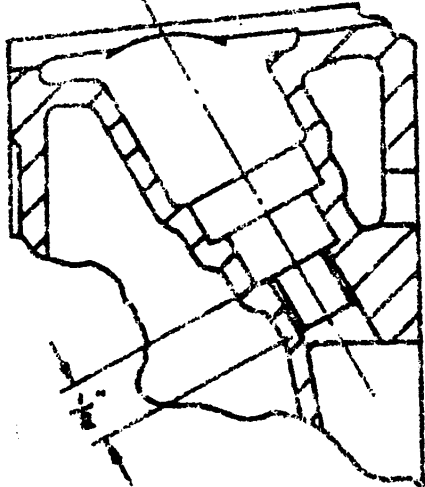
SPARK PLUG CAVITY TAPERED DIMENSIONS
