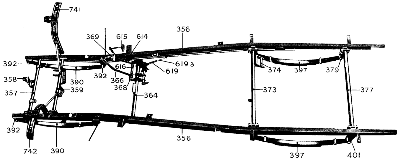
CHASSIS
