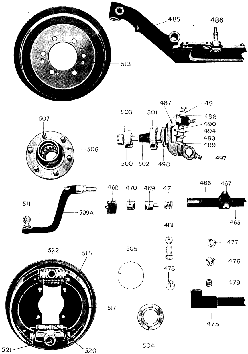
FRONT AXLE
